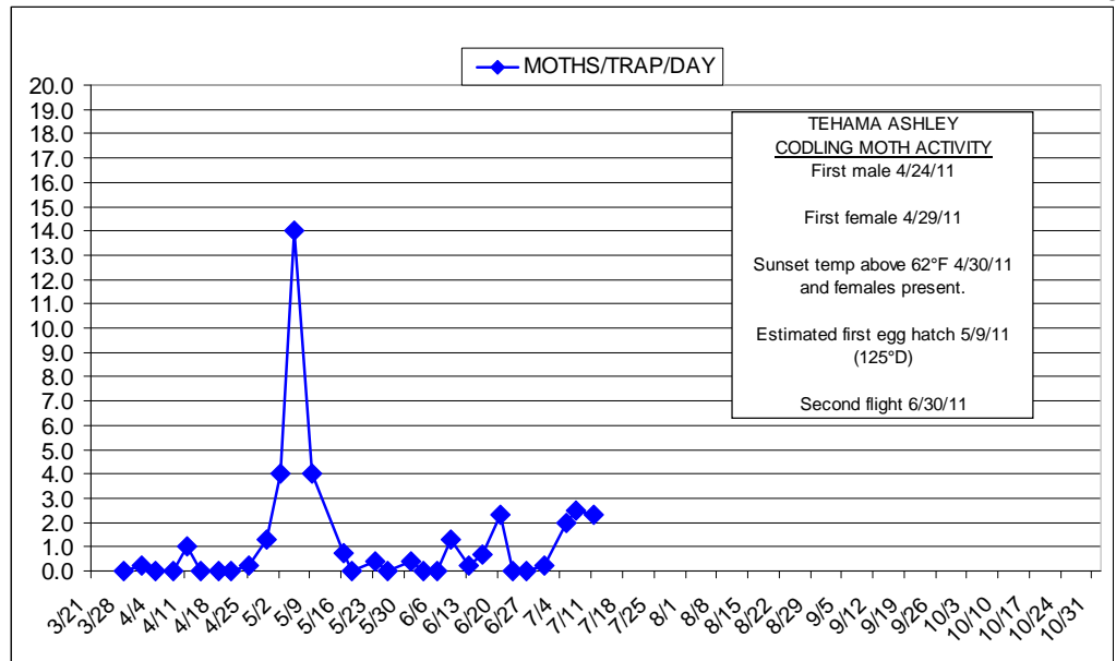
Figure 3. 2011 codling moth flight activity for Tehama County Ashley walnuts.
